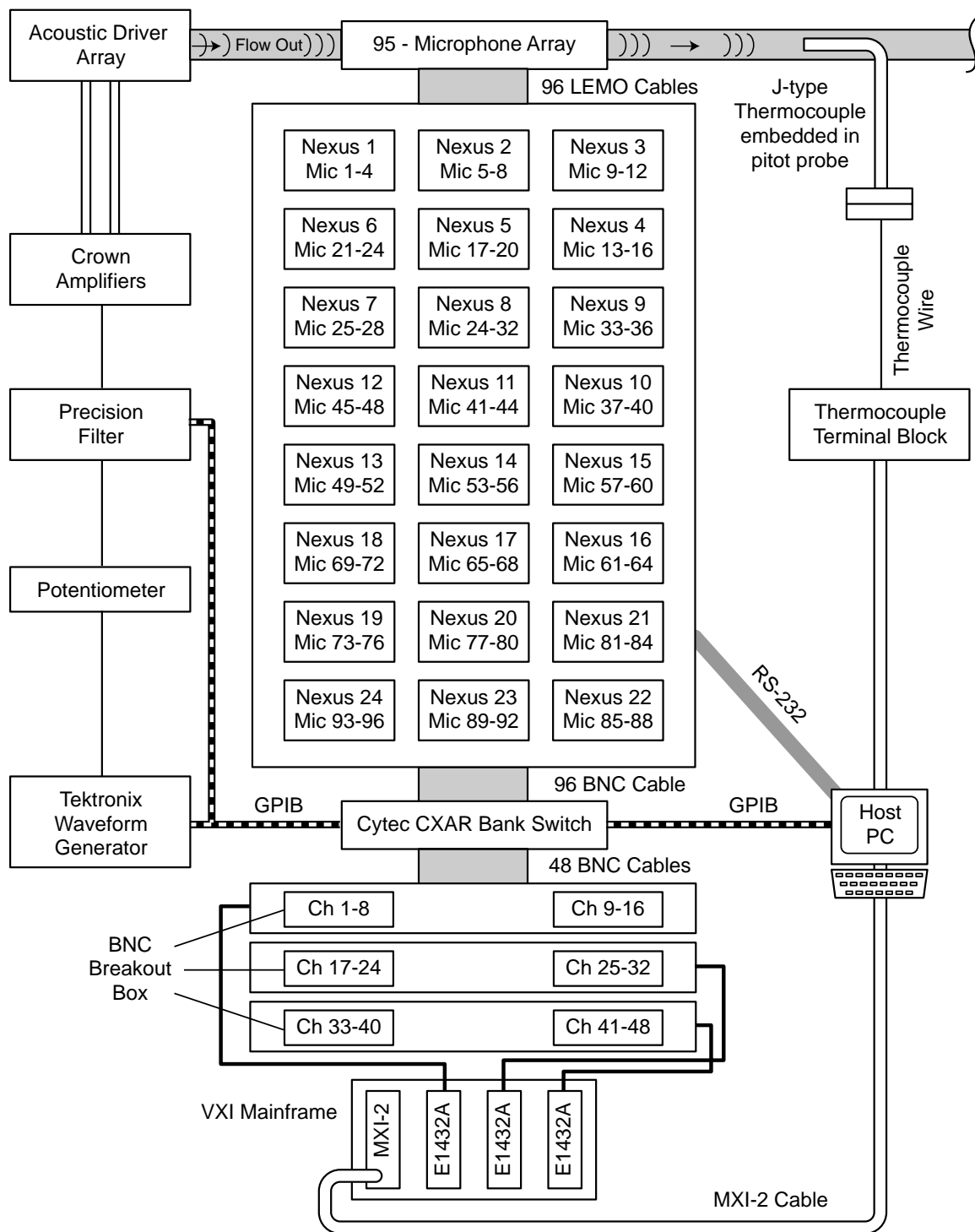
Figure 2. FIT Instrumentation Block Diagram.
